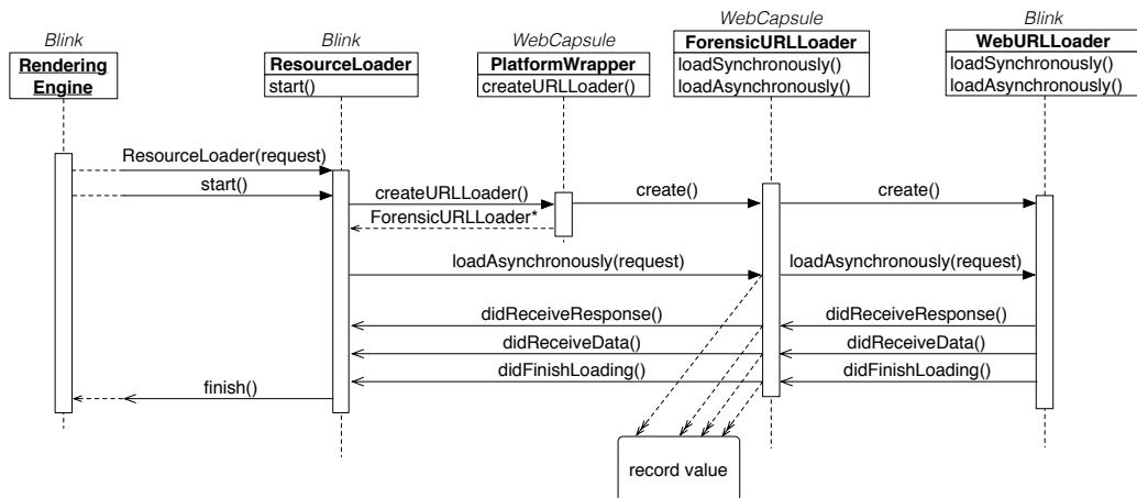
Figure 6: Simplified view of how WebCapsule records asynchronous network transactions.
